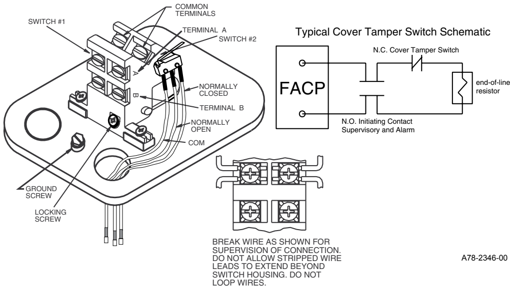
Figure 3. Switch terminals:
