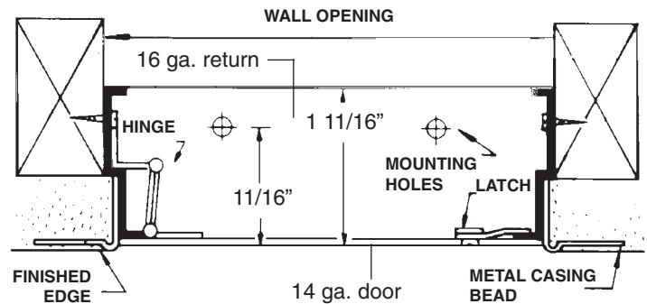
SECTION DETAIL
